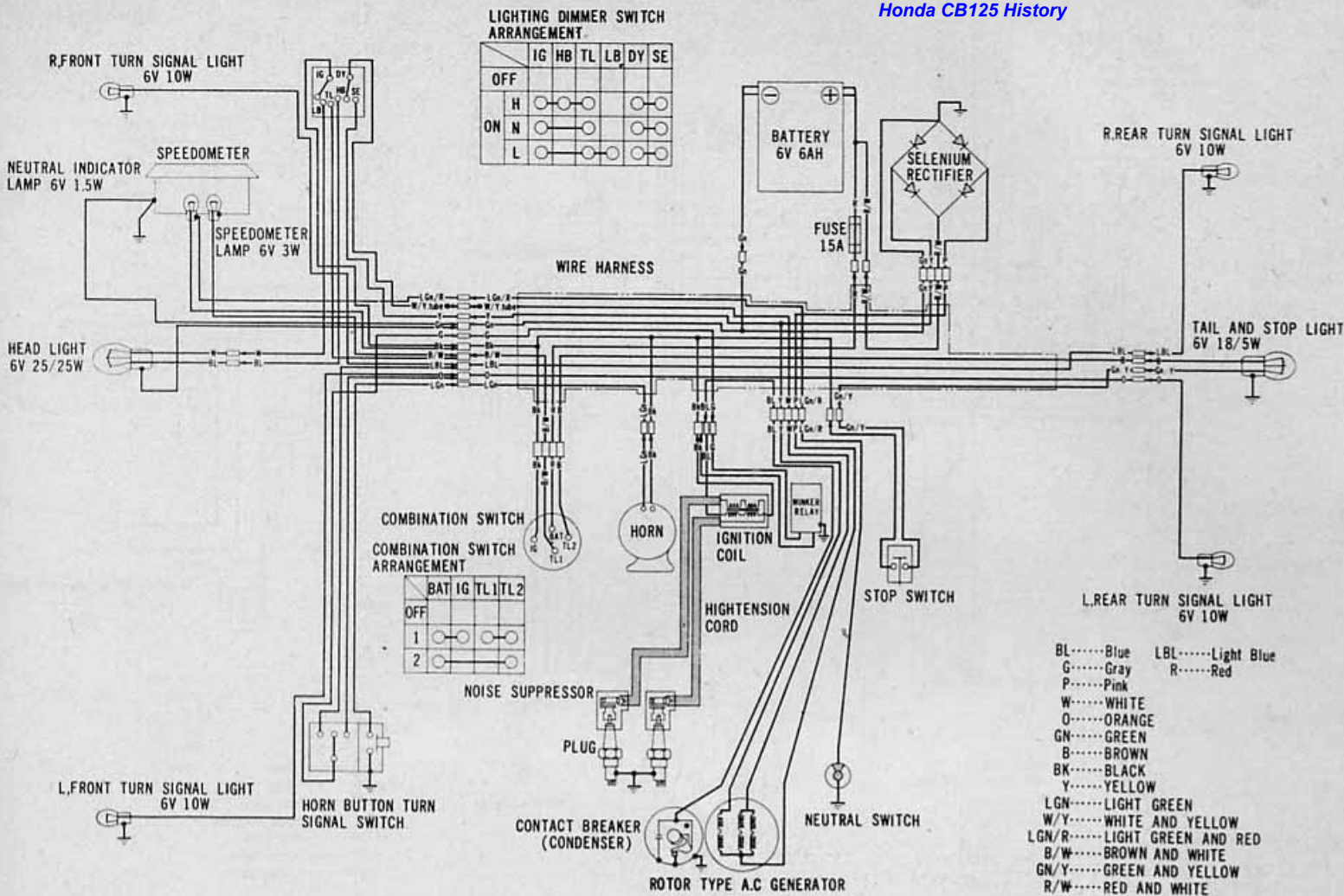
CB125 (early)
